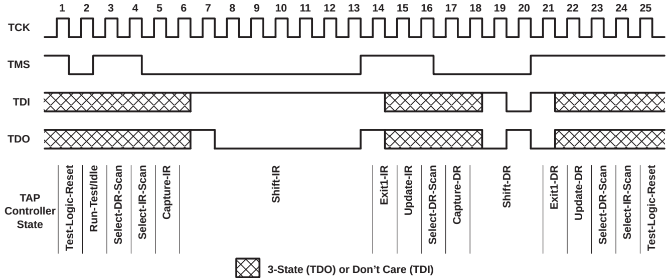
Figure 12. Timing Example
