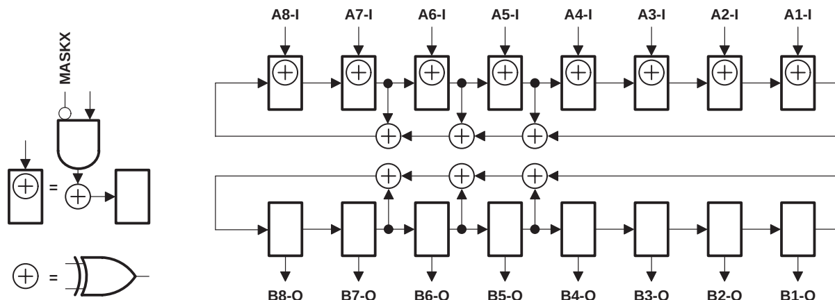
Figure 8. 8-Bit PSA/PRPG Configuration ( \overline{\text{OEAB}} = 0 , \overline{\text{OEBA}} = 1 )
