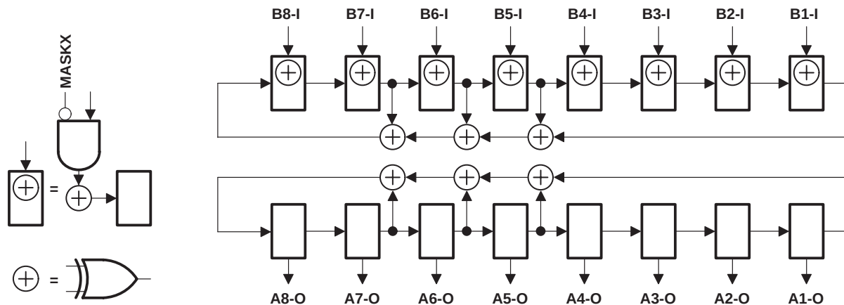
Figure 9. 8-Bit PSA/PRPG Configuration ( \overline{\text{OEAB}} = 1 , \overline{\text{OEBA}} = 0 )
